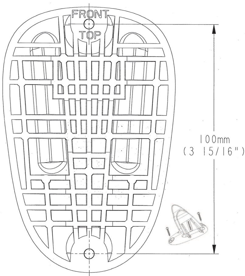
Figure 2. Drilling Template
