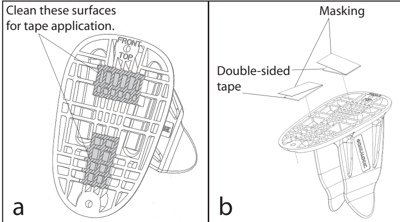
Figure 1. Applying the Double-Sided Tape
